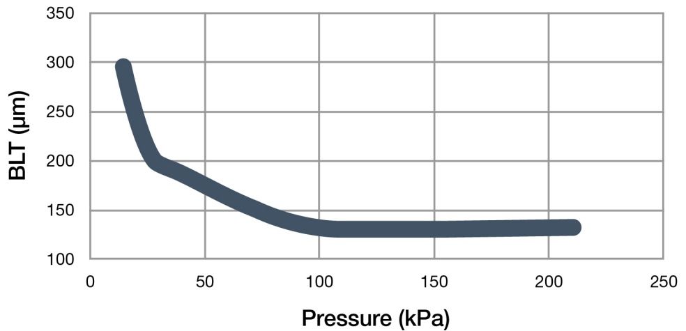
Figure 1: BLT of uncured DOWSIL™ TC-4060 Thermally Conductive Gel
