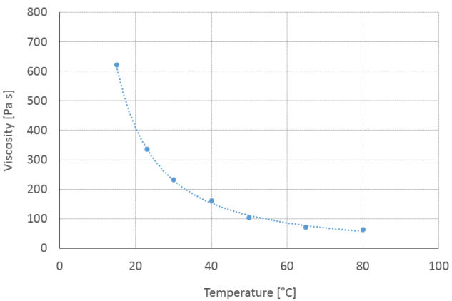
Fig. 1: VP 2106-408 Thermally Conductive Paste, viscosity vs. temperature (typical values).
